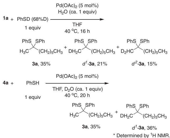
Scheme 3. The reaction using PhSD or D 2 O.
