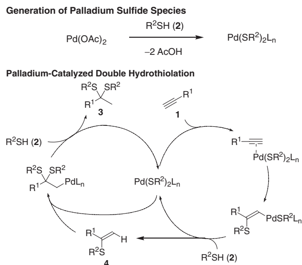
Scheme 2. A plausible reaction pathway.
