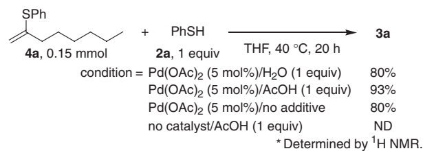
Scheme 1. Reactions of vinyl sulfide 4a .
